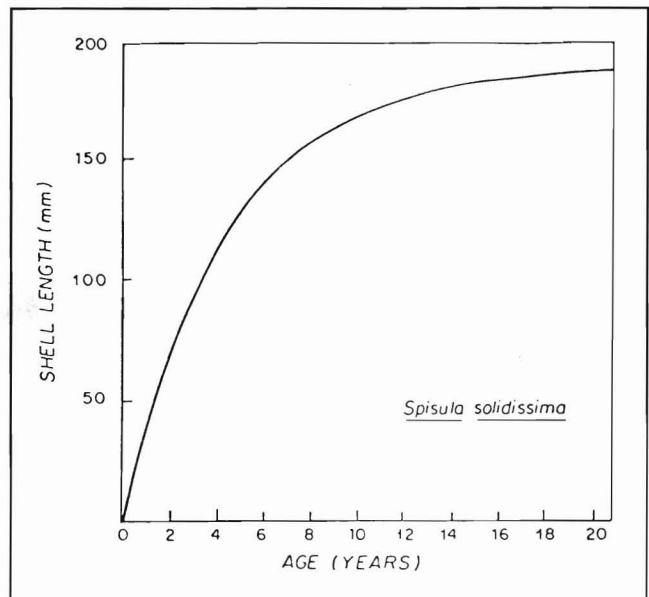
Figure 1 Relationship between age and growth in surf clams.
