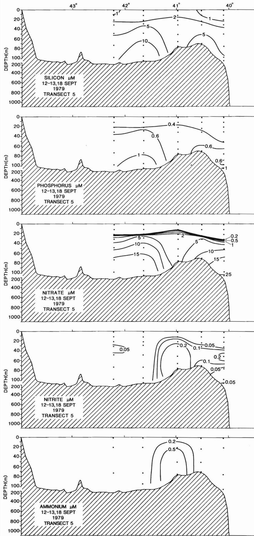
Figure 15.—Distribution of inorganic nutrients on Transect 5, 12-13, 18 September 1979.
