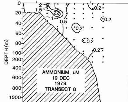
Figure 9.—Distribution of inorganic nutrients on Transect 8, 19 December 1979.
