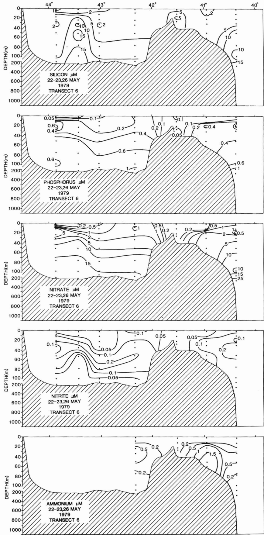
Figure 20.—Distribution of inorganic nutrients on Transect 6, 22-23, 26 May 1979.
