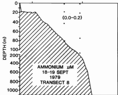
Figure 6.—Distribution of inorganic nutrients on Transect 8, 18-19 September 1979.
