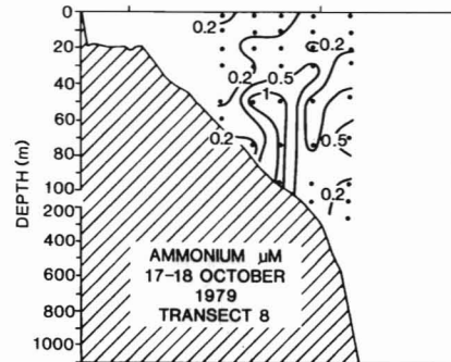
Figure 7.—Distribution of inorganic nutrients on Transect 8, 17-18 October 1979.
