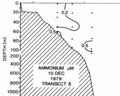
Figure 8.—Distribution of inorganic nutrients on Transect 8, 10 December 1979.
