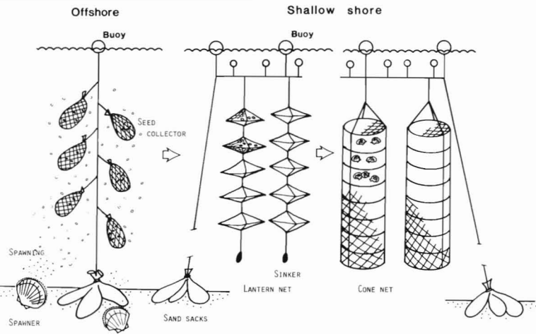
Figure 1.—Schematic representation of pecten culture. See text and Table 1 for explanation.
