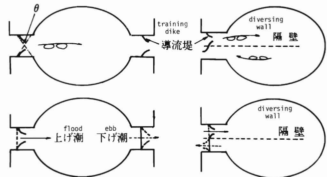
Figure 7.—Tidal current control by training dike.
