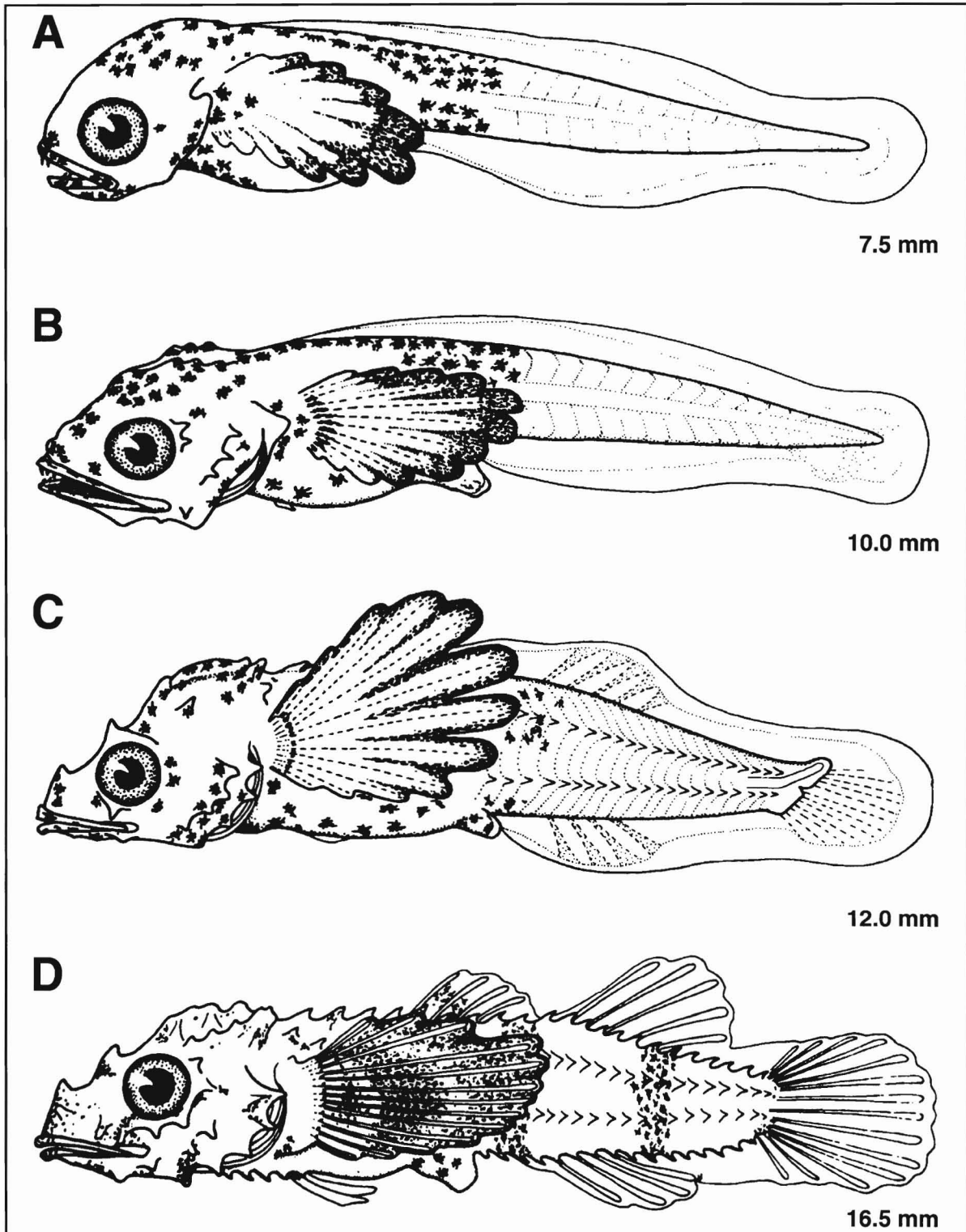
Figure 16 Developmental stages of Bothragonus swani (Marliave, 1975). (A) Preflexion larva 7.5 mm TL. (B) Preflexion larva 10.0 mm TL. (C) Flexion larva 12.0 mm TL. (D) Juvenile 16.5 mm TL.
