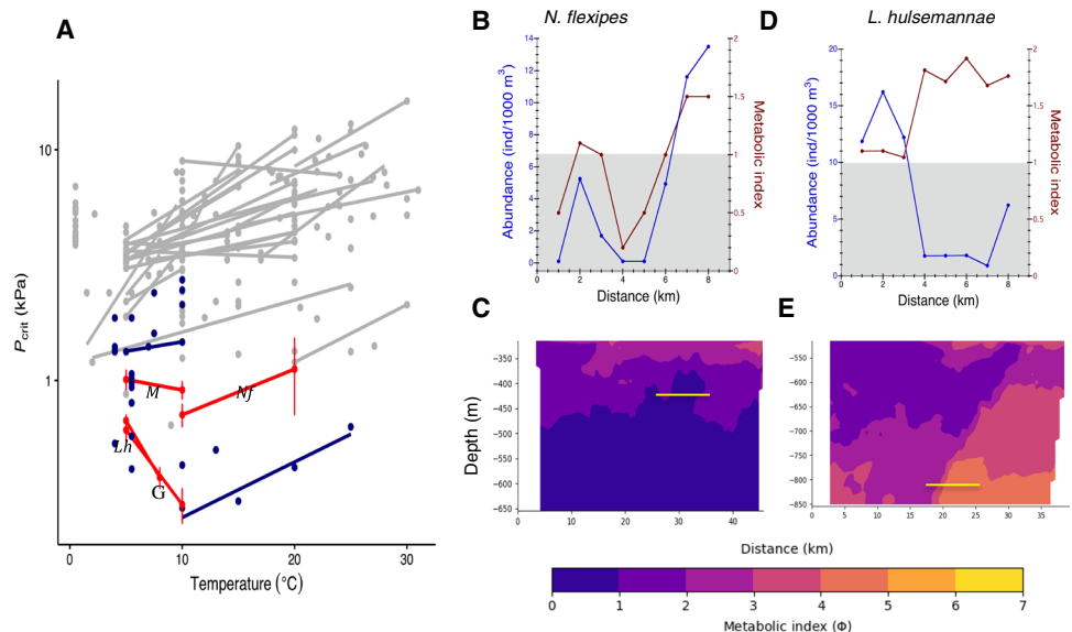
Fig. 5. Hypoxia tolerance influences the abundance of dominant mesopelagic crustaceans in the OMZ. (A) Critical PO_2 ( P_{crit} , kPa) in diverse marine crustaceans (gray; table S4), including species from the current study ( L. hulsemannae , Lh ; N. flexipes , Nf ; Gennadas spp., G ; and Megacalanus spp., M ; red, means \pm SE; table S3) and from the eastern Pacific OMZ (blue). Lines connect intraspecific measurements at different temperatures. Note that the y axis is on a log scale. (B to E) MI calculated for N. flexipes (B and C) at 400 m and L. hulsemannae (D and E) at 800 m from metabolic and environmental data across the horizontal MOCNESS [red lines in (B) and (D)] and Wire Flyer transects (C and E). The yellow line on MI plots illustrates the corresponding MOCNESS tows. The corresponding abundance of each species is also plotted [blue lines in (B) and (D)]. Gray shading (B and D) indicates metabolically unavailable habitat (MI < 1).
