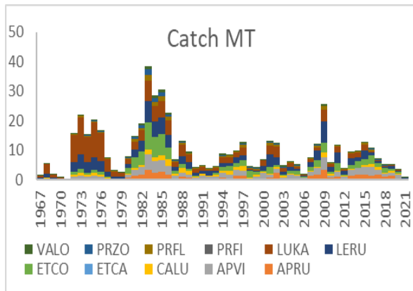
Figure 2: Species-based landings
