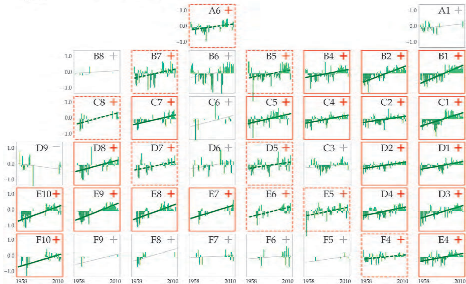
Figure 10.3 Spatio-temporal trends plot for Phytoplankton Colour Index time-series in the CPR standard areas of the North Atlantic Basin based on data for 1958–2010.
