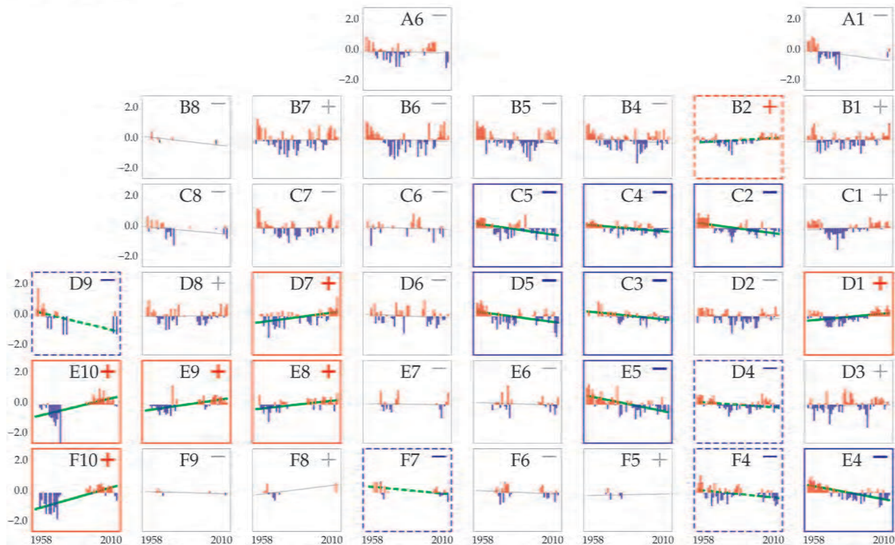
Figure 10.5 Spatio-temporal trends plot for Total Diatoms time-series in the CPR standard areas of the North Atlantic Basin based on data for 1958–2010.
