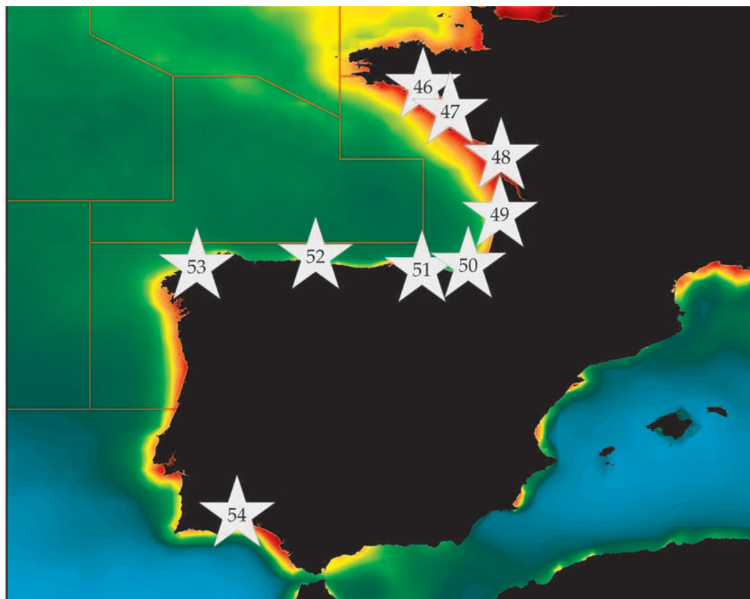
Figure 8.1 Locations of the Bay of Biscay and western Iberian Shelf plankton monitoring areas (Sites 46–54) plotted on a map of average chlorophyll concentration.
