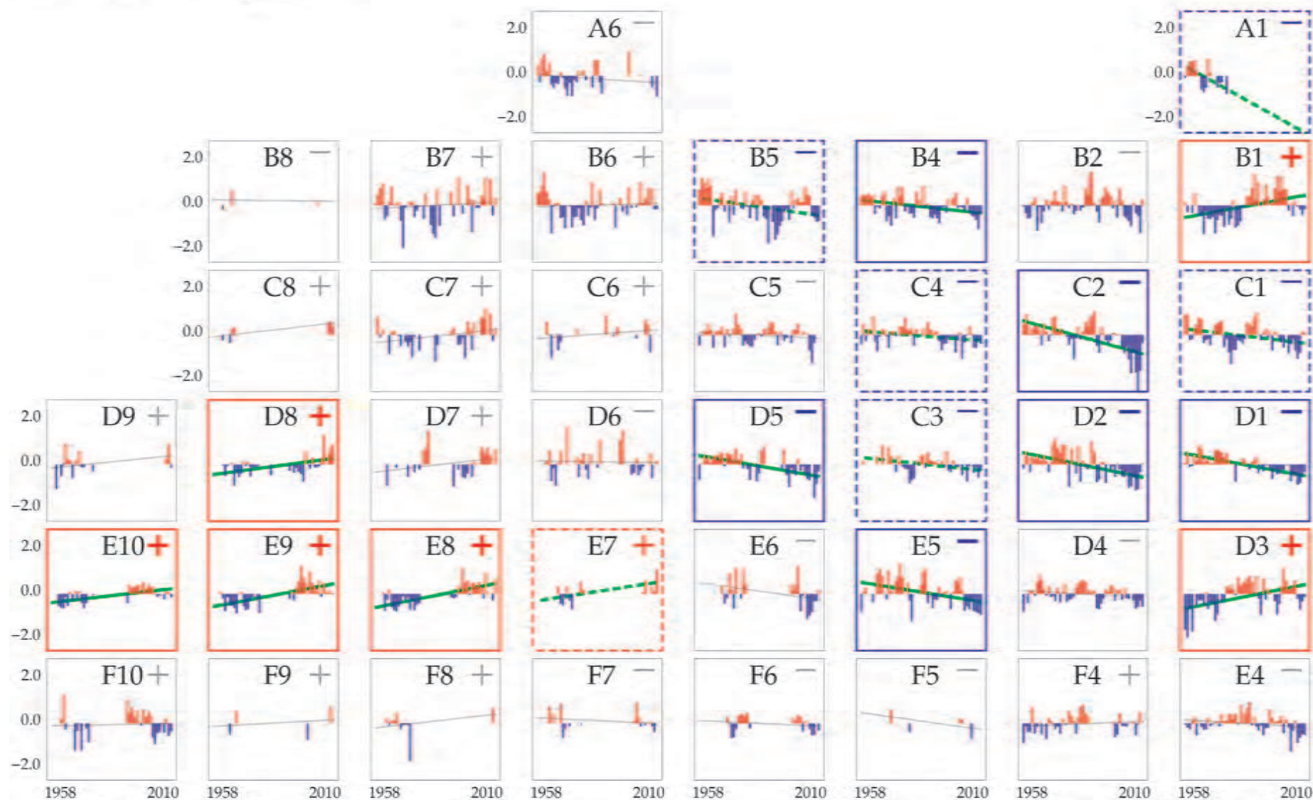
Figure 10.6 Spatio-temporal trends plot for Total Dinoflagellates time-series in the CPR standard areas of the North Atlantic Basin based on data for 1958–2010.
