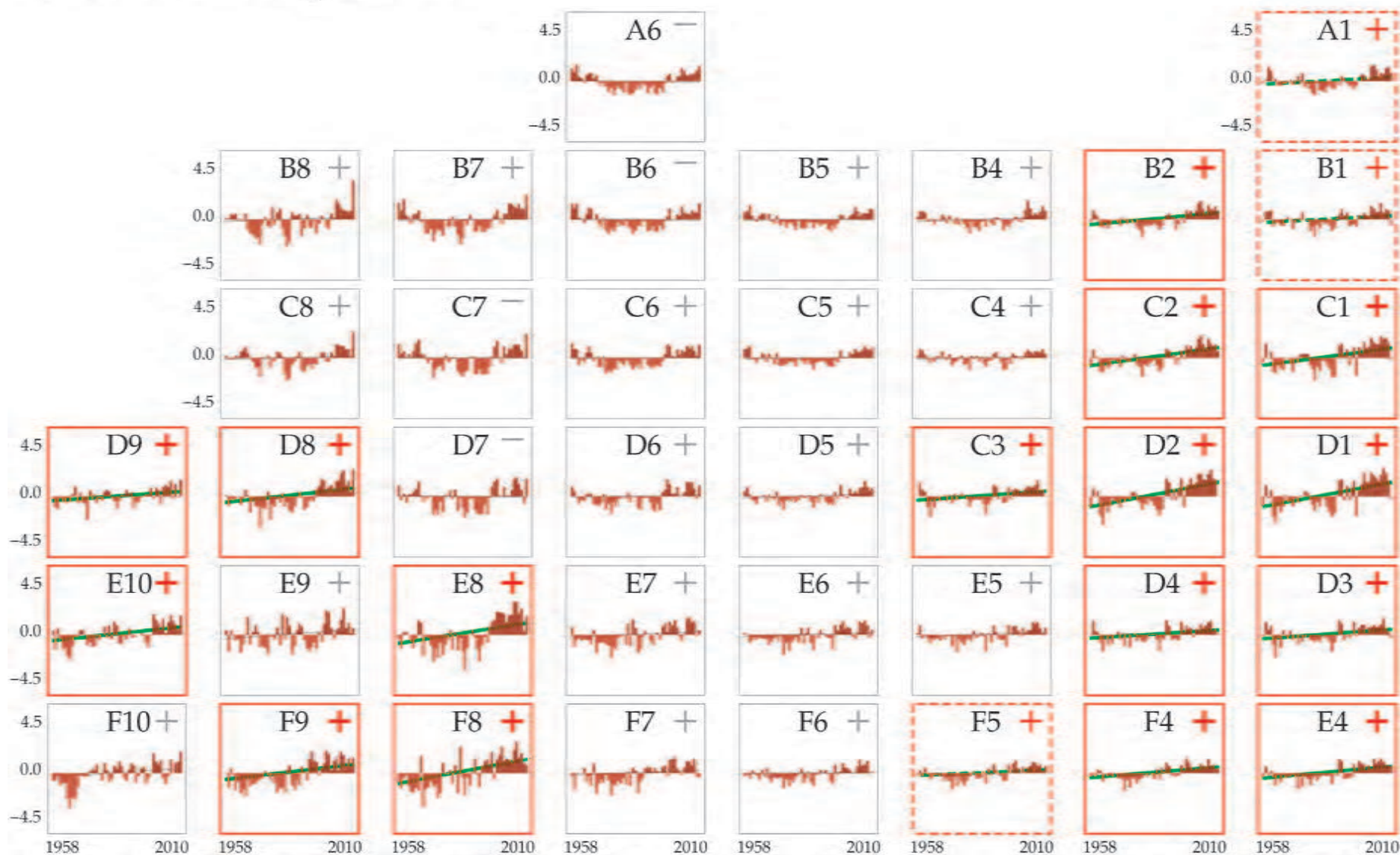
Figure 10.4 Spatio-temporal trends plot for sea surface temperature time-series in the CPR standard areas of the North Atlantic Basin based on data for 1958–2010.
