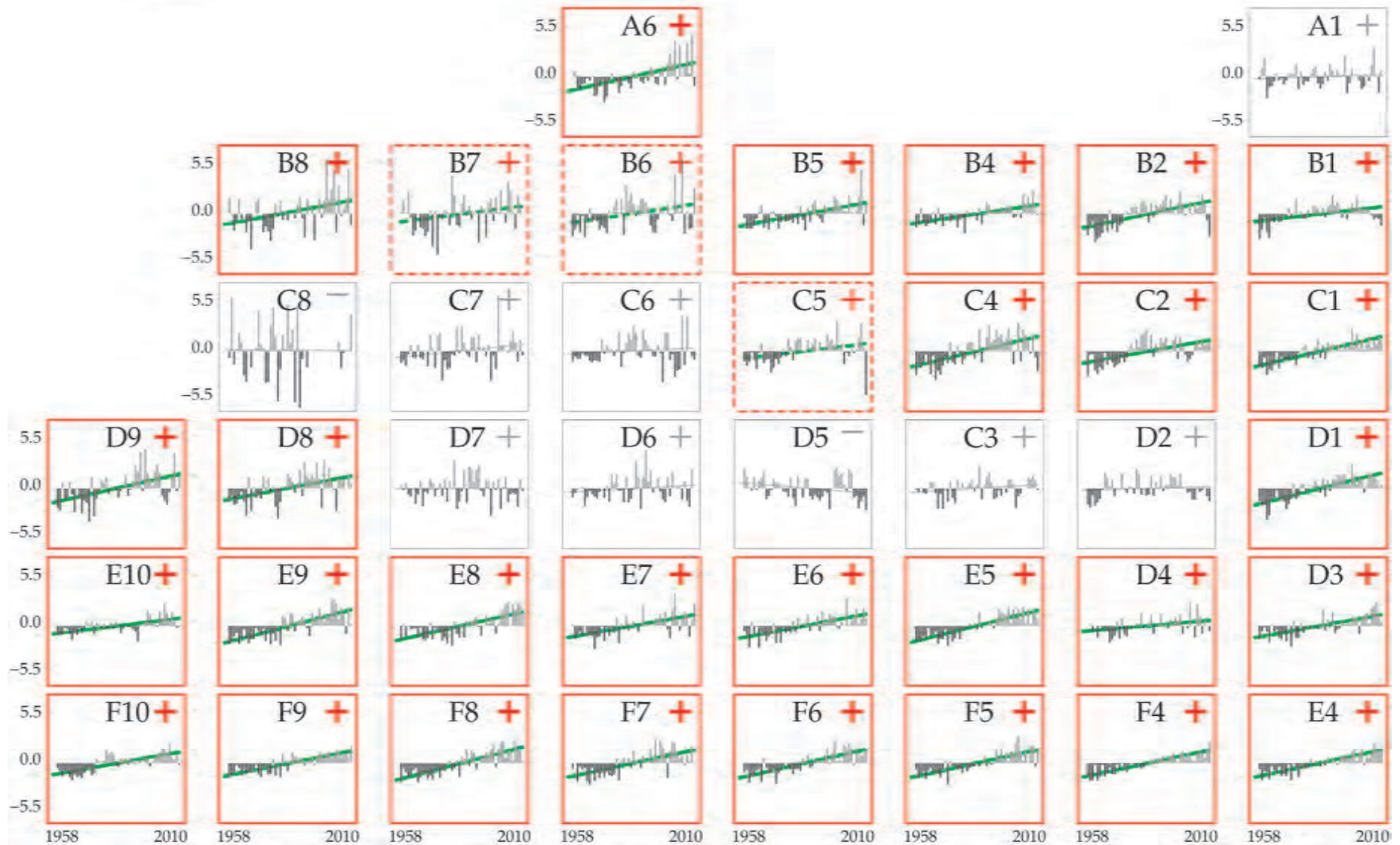
Figure 10.8 Spatio-temporal trends plot for COADS Wind speed time-series in the CPR standard areas of the North Atlantic Basin based on data for 1958–2010.
