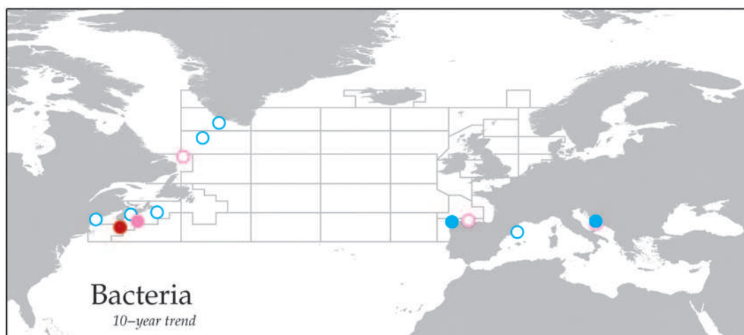
Figure 11.10 Spatio-temporal map of 10-year trends in bacteria abundance present within the phytoplankton monitoring sites. (This variable is not currently available from the CPR programme.) Symbol colors indicate slope (blue/cyan = negative, red/pink = positive) and statistical significance (dark red/blue = p < 0.01 , pink/cyan = p < 0.05 ). Symbols with a white, unfilled, centre indicate slope with a non-significant ( p > 0.05 ) trend.
